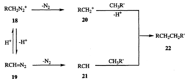
Scheme 6. Possible reaction paths to form the insertion product.
